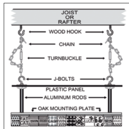
Over-the-Counter Display Tile Mounting
